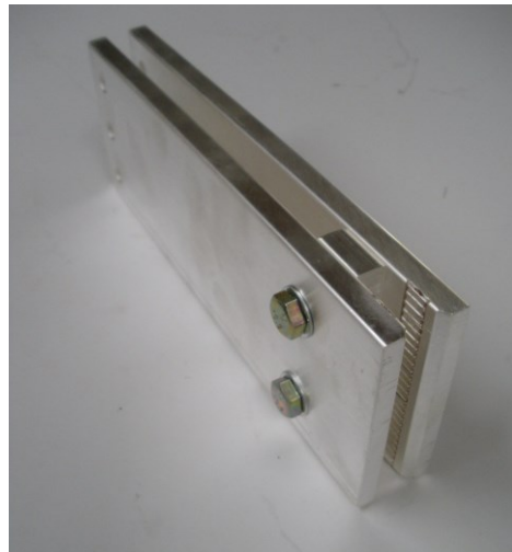
Connection plate for permanent extension of 10mm thick main busbars (approx 3500A)
